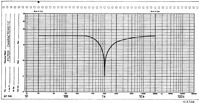
Fig. 9.3. Output from the Level Recorder.
