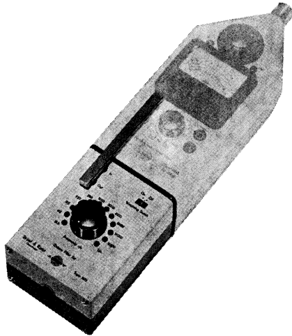
Fig. 3.1. The Octave Filter Set Type 1613 joined to the Sound Level Meter.
