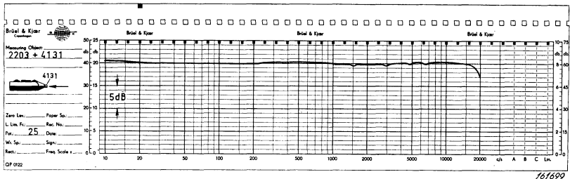
Fig. 6.5. Frequency response of the instrument with microphone Type 4131.
