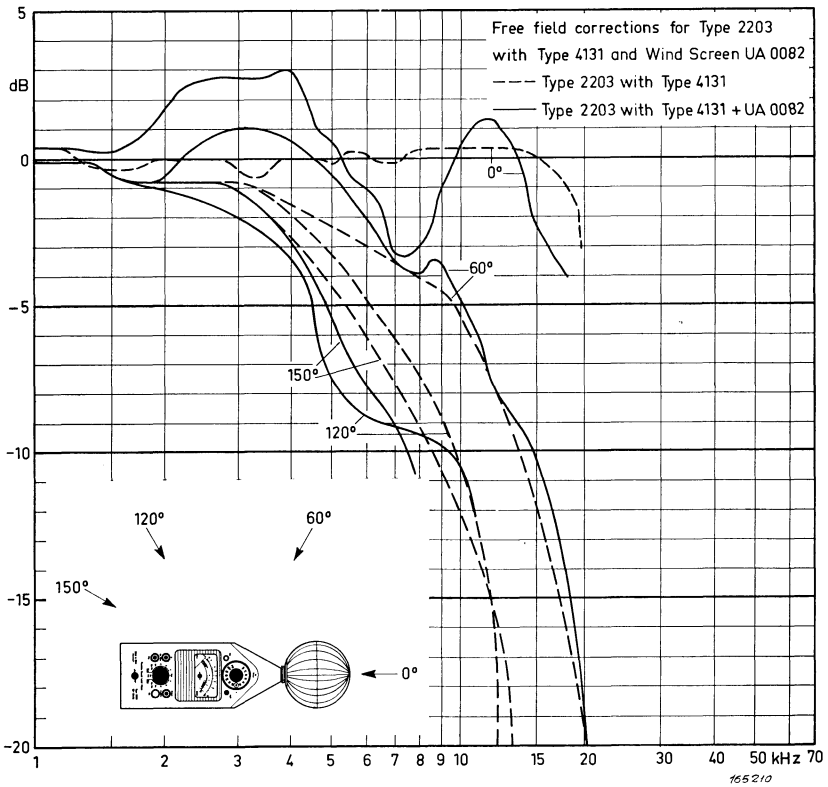
Fig. 8.8. Correction curves for 0°, 60°, 120° and 150° angles of incidence.
