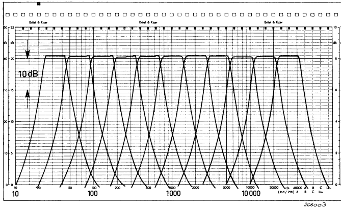
Fig. 3.3. Complete set of filter characteristics for Type 1613.
