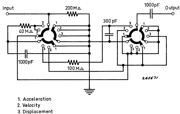
Fig. 4.3. Circuit diagram for the Integrator ZR 0020.
