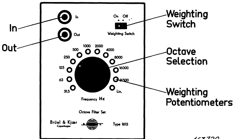
Fig. 4.2. The Octave Filter Set Type 1613.
