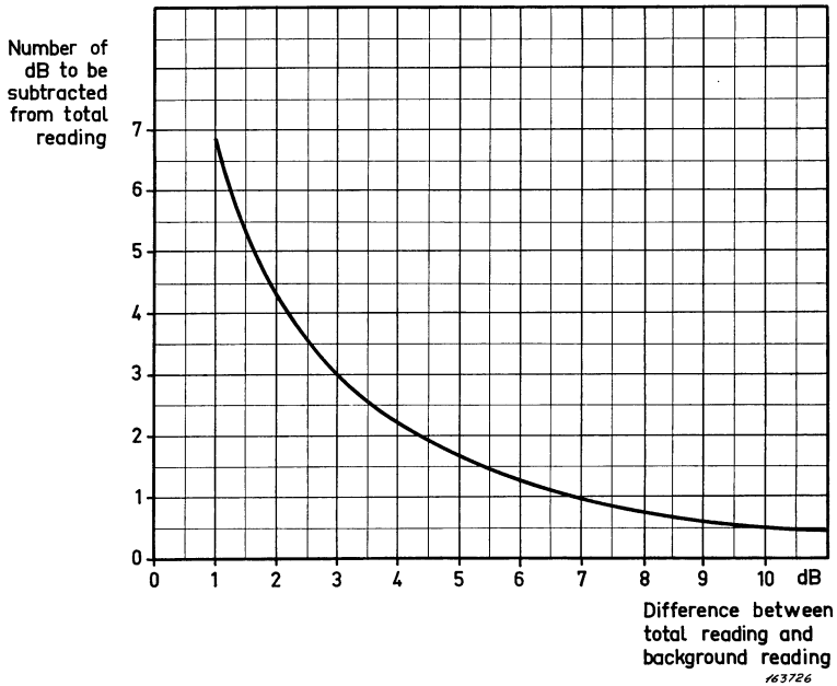
Fig. 6.8. Background correction.
