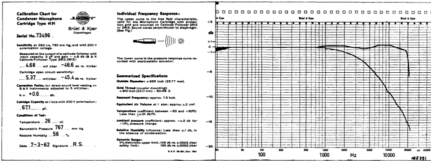
Fig. 5.1. Typical calibration chart as supplied with the microphone cartridges. The automatic plotting process used in production has an accuracy of 0.2 dB up to 10 kHz and 0.5 dB up to 20 kHz.
