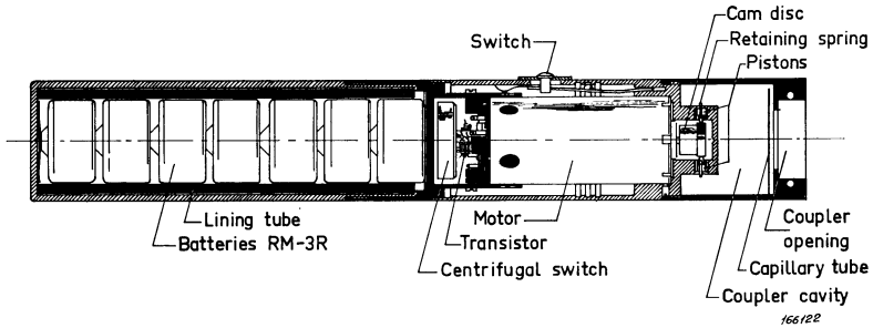
Fig. 7.2. Assembly drawing of the Pistonphone.
