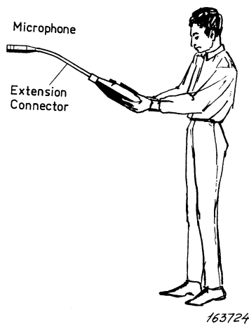
Fig. 6.6. Sound Level Meter with Extension Connector.
