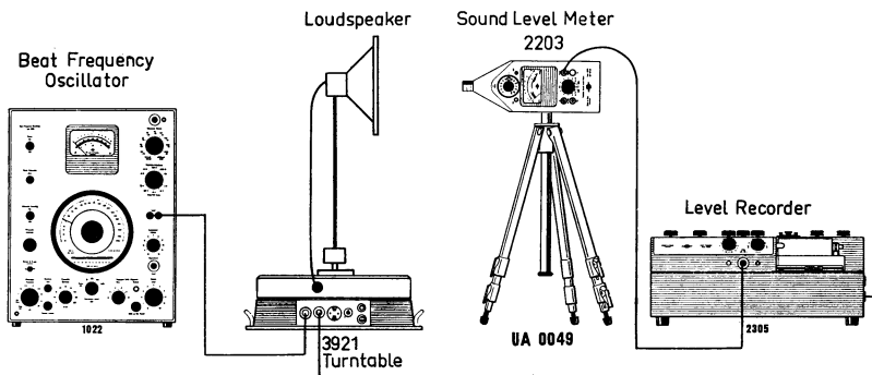
Fig. 9.5. Set-up for finding frequency response and directivity pattern of a loudspeaker.
