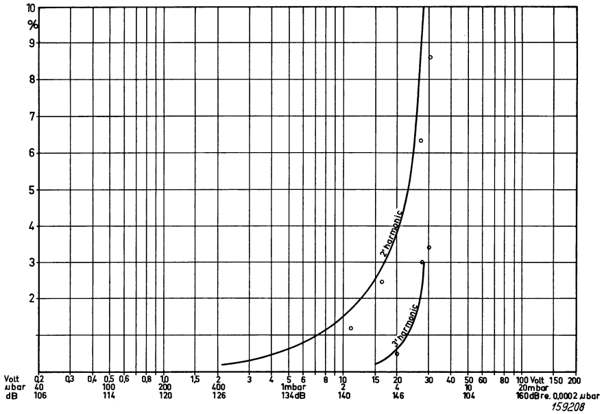
Fig. 5.9. Typical distortion curves for the one-inch microphones. The curves in full are measured on the source-follower and referred to a complete microphone with a sensitivity of 5 mV/ \mu bar. The measuring points shown are averages measured in a pistonphone on a number of complete microphones at 50 Hz.
