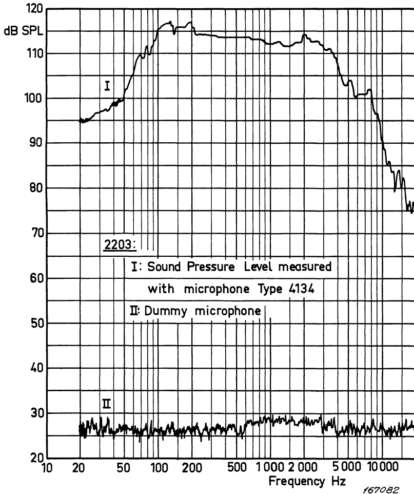
Fig. 5.7. The Sound Level Meter exposed to a sound field of approximately 120 dB. Curve I shows the sound pressure level, and curve II shows the output of the Sound Level Meter when the microphone was replaced with an equivalent impedance.
