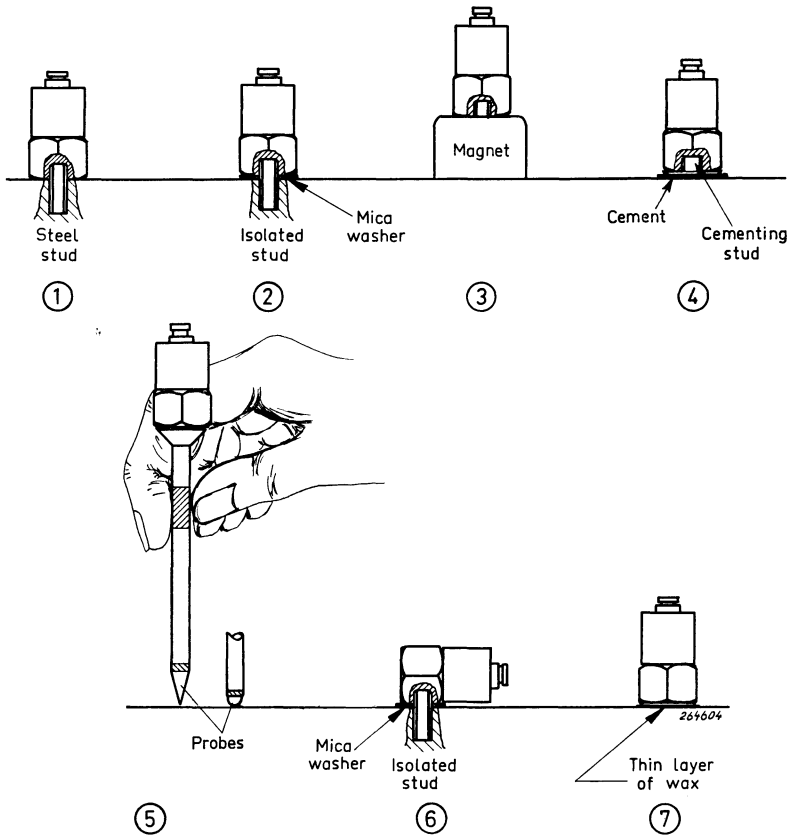
Fig. 9.1. Different ways of mounting the Accelerometer.
